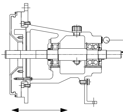
Fig. 2 Shaft axial clearance.
