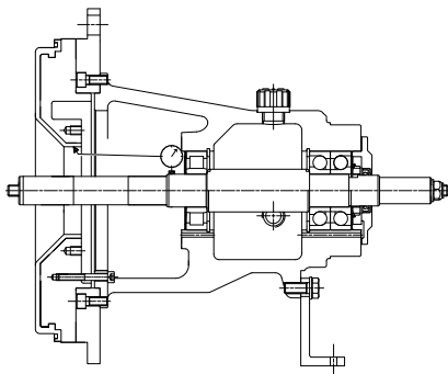
Fig. 4 Concentricity between shaft and stuffing box housing.
