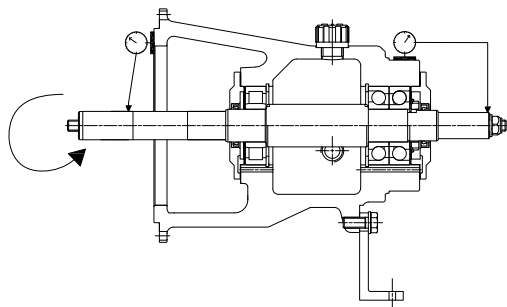
Fig. 1 Shaft radial oscillation.
