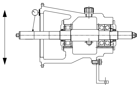
Fig. 3 Shaft radial clearance.
